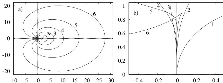
Figure 1: a) Absolute stability regions of the BDF up to order six with constant stepsize. The regions are the exterior of the closed curves. b) Detail close to the origin.
