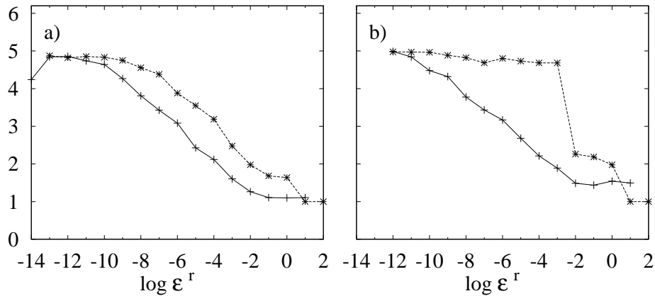
Figure 4: (a), (b) The average order, k_{av} , versus the logarithm of the relative tolerance, \log \varepsilon^r , for the semi-implicit VSVO methods, and the C_1 and C_2 cases, respectively. The symbols mean: Q -explicit VSVO (+, solid line), and Q -implicit VSVO (*, dashed line). The vertical axis is the same for the two plots.
