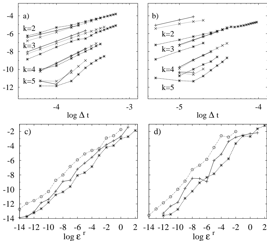
Figure 2: (a) \log \varepsilon(u) versus \log \Delta t for constant stepsize integration, k from 2 to 5, in the C_1 case. (c) \log \varepsilon(u) versus \log \varepsilon^r for the VSVO methods in the C_1 case. (b), (d) Same as (a) and (c), respectively, for the C_2 case. The symbols mean: Q -explicit (+, solid line), Q -splitting ( \times , dotted line), Q -implicit (*, dashed line), Q -explicit VSVO (+, solid line), Q -implicit VSVO (*, dashed line) and DLSODPK (o, dash-dotted line). The vertical axis is the same in each row of plots.
