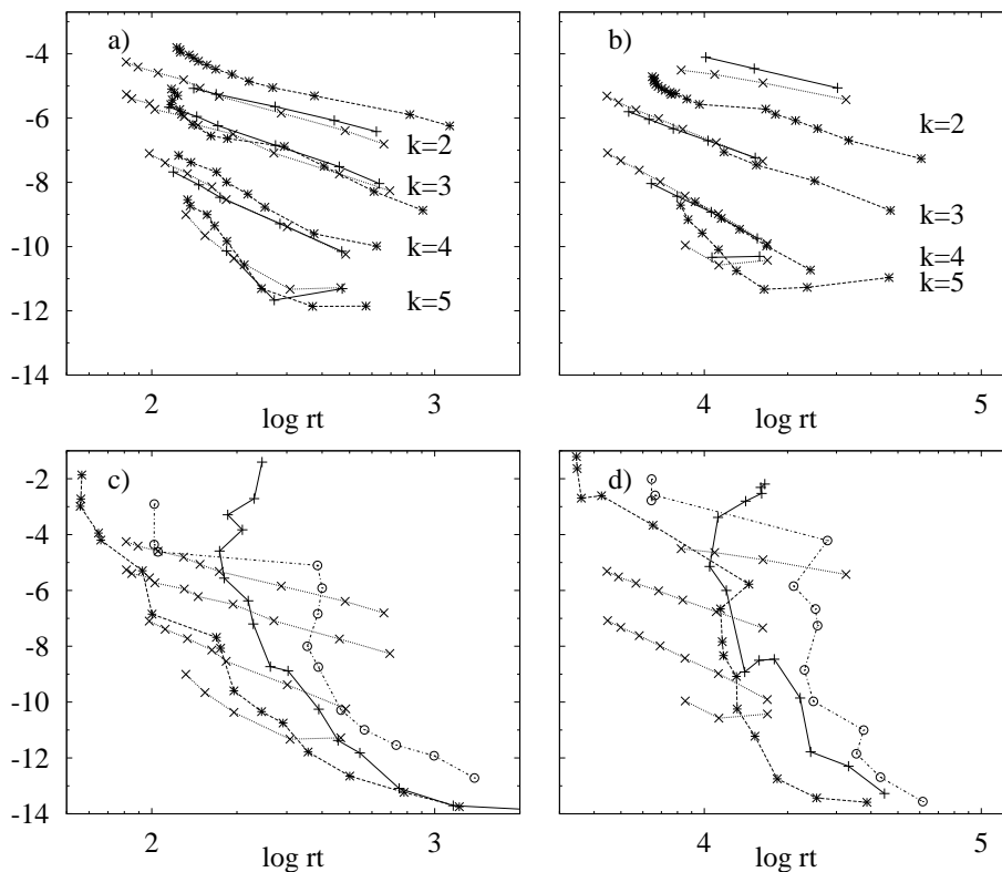
Figure 3: (a) \log \varepsilon(u) versus the logarithm of the run time, \log rt , for constant stepsize integration, k from 2 to 5, in the C_1 case. (c) Same as (a) for the Q -splitting and VSVO methods. (b), (d) Same as (a) and (c), respectively, in the C_2 case. The symbols mean: Q -explicit (+, solid line), Q -splitting ( \times , dotted line), Q -implicit ( * , dashed line), Q -explicit VSVO (+, solid line), Q -implicit VSVO ( * , dashed line), and DLSODPK ( \circ , dash-dotted line). The vertical axis is the same in each row of plots.
