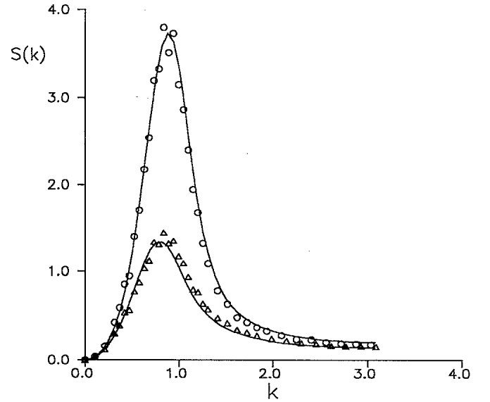
FIG. 1. Evolution of the structure function for a very small time \tau=5 . Circles and triangles correspond to numerical simulation of Eq. (4.11) with c^3=0 , for a=0 and a=0.8 , respectively. The lines correspond to the numerical integration of Eq. (4.13) for the same values of a ( \beta^{-1}=0.3 ).
