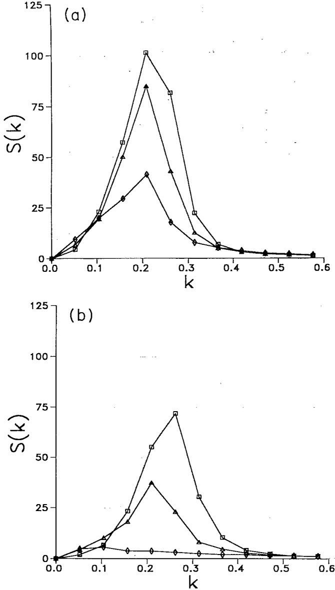
FIG. 4. Structure function obtained from Eq. (4.11) at \tau=1500 for (a) a=0 and (b) a=0.8 . Squares, \beta^{-1}=0.1 ; triangles, \beta^{-1}=0.2 and rhombus, \beta^{-1}=0.3 .
