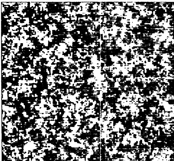
FIG. 2. Typical configurations obtained from Eq. (4.11) at \tau=500 , starting from an homogeneous situation, c=0 , for \beta^{-1}=0.3 and (a) a=0 and (b) a=0.8 .
