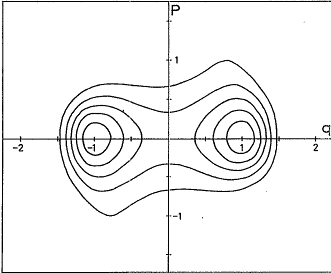
FIG. 1. Contours representing loci of constant probability corresponding to P_{st}(q, p) of Eqs. (3.10) and (3.15)–(3.18) for \lambda=1 , D=0.3 , and \tau=0.5 .
