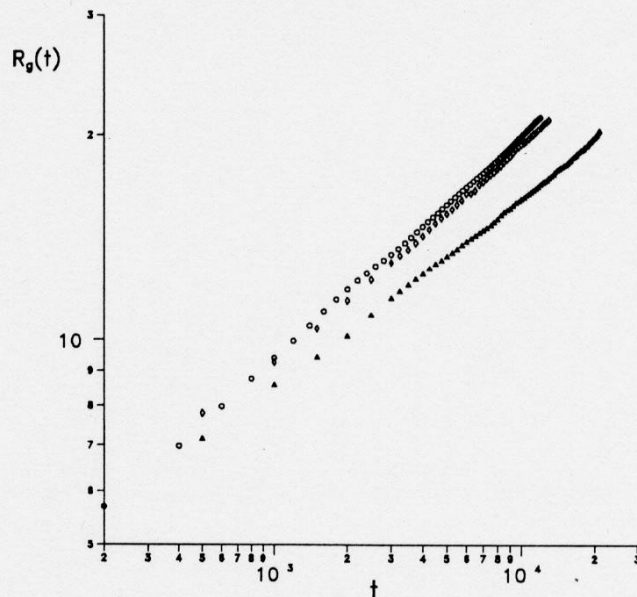
Fig. 1. log-log plot of the time evolution of R_g(t) for a deterministic system (o) and for a system with additive noise ( \diamond ) and with multiplicative noise ( \triangle ).
