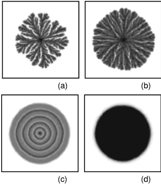
FIG. 5. Patterns obtained for n_0=1 with D_0=0.025 (a) and D_0=0.05 (b) and for n_0=5 with D_0=0.05 (c) and D_0=1 (d). They correspond to times t=500 , 300, 50, and 25, respectively.
