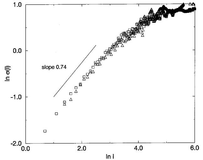
FIG. 4. Width of the rough interface as a function of the length of the interval in which it is measured. They correspond to the pattern of Fig. 2(b) ( \square ) and to a case with the same parameters but with strip geometry ( \triangle ). A line of slope 0.74 is also plotted for comparison with experimental results.
