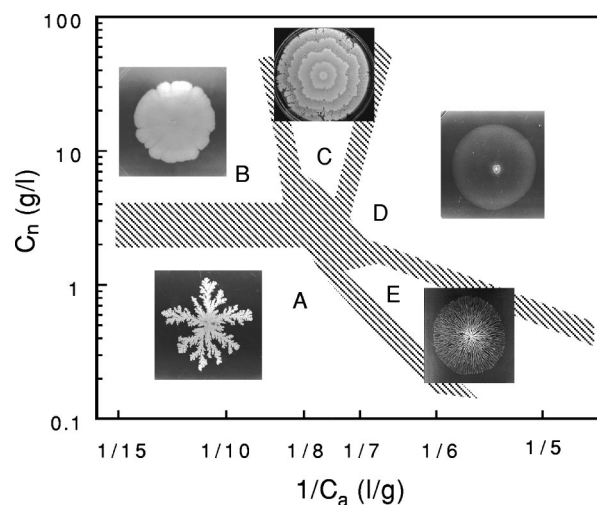
FIG. 1. Morphological diagram of patterns observed in colonies of Bacillus subtilis OG-01 as a function of nutrient concentration ( C_n ) and the hardness of agar surface ( 1/C_a , C_a being the agar concentration). Experiments were performed in a Petri dish with a diameter of 88 mm. Taken with permission from [8].
