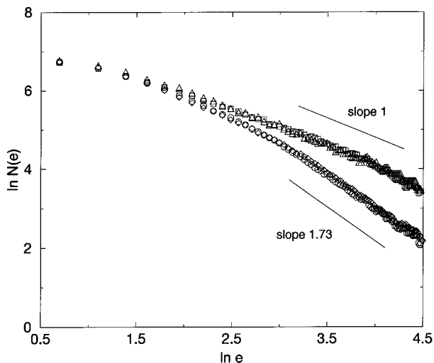
FIG. 3. Fractal dimensions determined by the box-counting method, for D_0=0.005 and n_0=1 ( \circ ), 2 ( \diamond ), 3 ( \square ), and 5 ( \triangle ). Two lines of slopes 1 and 1.73 are also plotted for comparison with experiments.
