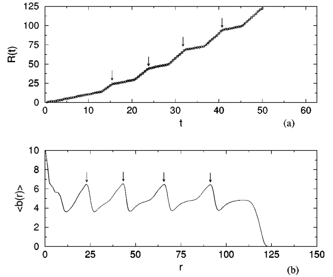
FIG. 6. (a) Time evolution of the colony radius, for parameters D_0=0.05 and n_0=5 ; (b) radial density profile corresponding to time t=50 [pattern of Fig. 5(c)]. The positions where each consolidation phase started are pointed out.
