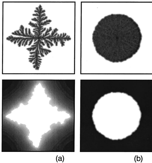
FIG. 2. Bacterial colonies (top) and nutrient patterns (bottom) for a fixed value of D_0=0.005 and two values of initial nutrient: n_0=1 (a) and n_0=5 (b). They correspond to times t=2500 and 75 , respectively.
