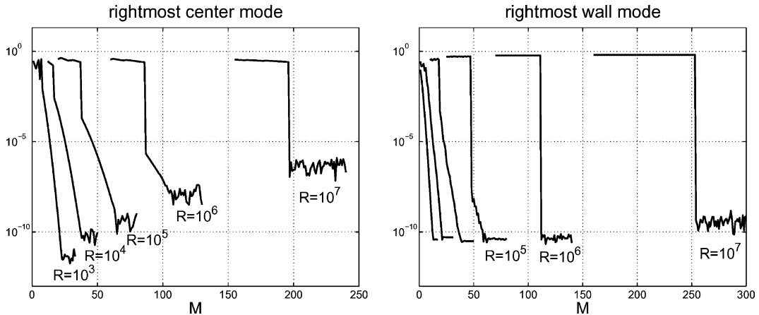
Fig. 2. Error in the rightmost center and wall mode eigenvalues as a function of discretization parameter M , for n = 0 and k = 1 and Reynolds numbers R = 10^2, 10^3, \dots, 10^7 . The matrix dimension is 2M + 2 . The convergence is spectral in each case until limited by rounding errors. As R \rightarrow \infty , the value of M needed to resolve these modes is about R^{1/3} .
