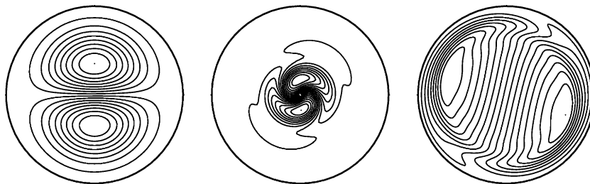
Fig. 4. Stream functions of the same three modes as in Fig. 3 for R = 3000 . The angular orientation is arbitrary.
