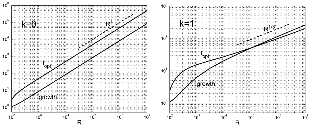
Fig. 6. Dependence of \sup_t \|\exp(t\mathcal{L})\| and t_{opt} on R for n = 1 and k = 0, 1 .
