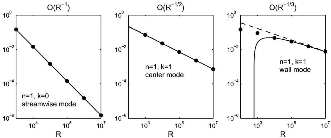
Fig. 3. (Negatives of) real parts of rightmost eigenvalues as a function of R for n = 1, k = 0 (streamwise modes) and n = 1, k = 1 (center modes, wall modes). The solid curves show the approximations (31)–(33). The dashed curves in the second and third plots (barely visible in the second plot) correspond to just the first terms of these approximations.
