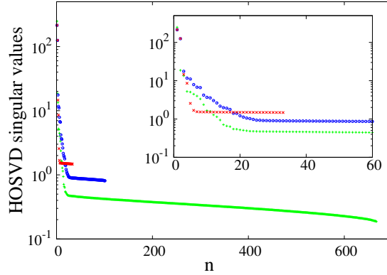
Figure 15: HOSVD singular values along the radial (red), azimuthal (blue), and temporal (green) directions.
