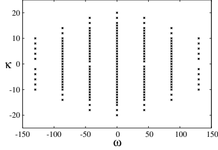
Figure 7: The \kappa - \omega diagram for the more complex period flow.
