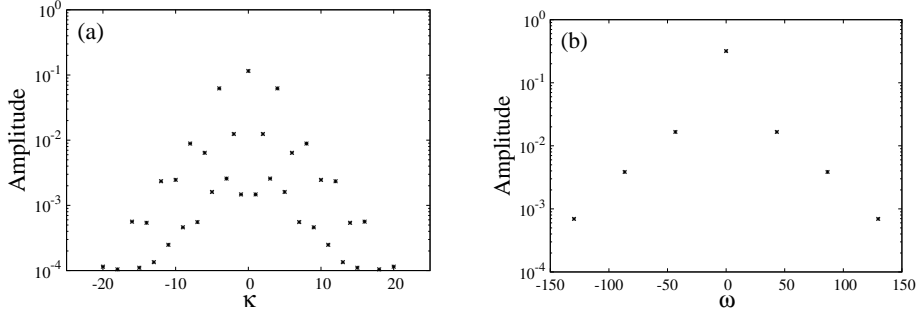
Figure 8: The (a) a - \kappa and (b) a - \omega diagrams for the more complex period flow.
