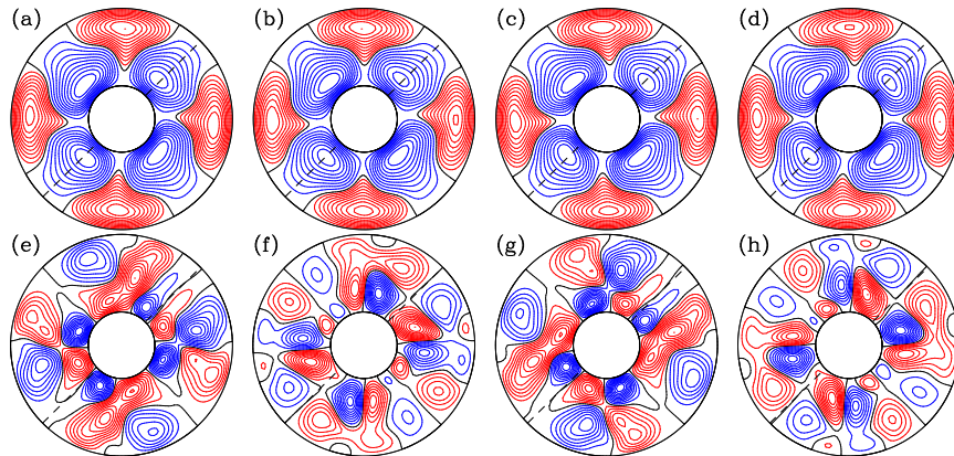
Figure 5: Counterpart of Fig. 1 for the more complex periodic flow.
