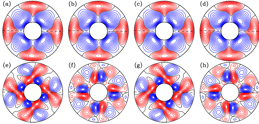
Figure 1: Four representative snapshots of the perturbation of the temperature for the simple periodic flow at (a) t = 0 , (b) t = T/4 , (c) t = T/2 , and (d) 3T/4 , with the exact symmetry diameter (as computed below, see Eq. (3.19)) indicated with thick dashed line. (e–h) same snapshots after subtracting the mean field.
