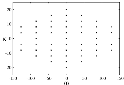
Figure 3: The \kappa - \omega diagram for the simple periodic flow.
