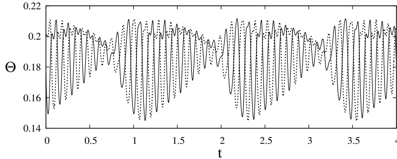
Figure 10: Counterpart of Fig. 2 for the quasi-periodic flow.
