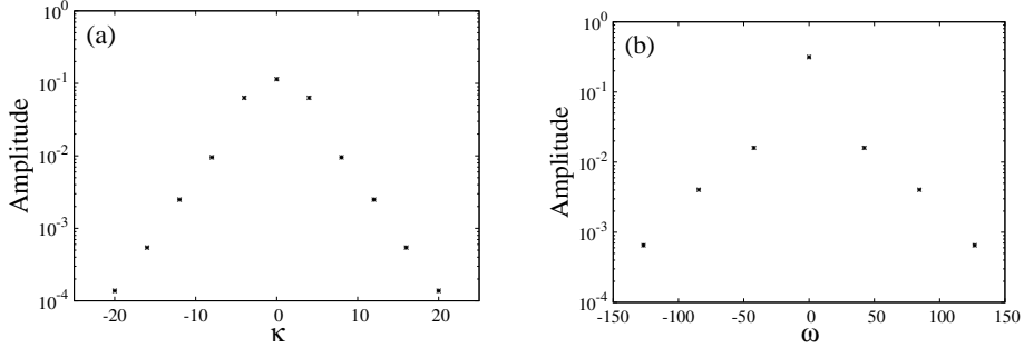
Figure 4: The (a) a - \kappa , and (b) a - \omega diagrams for the simple periodic flow.
