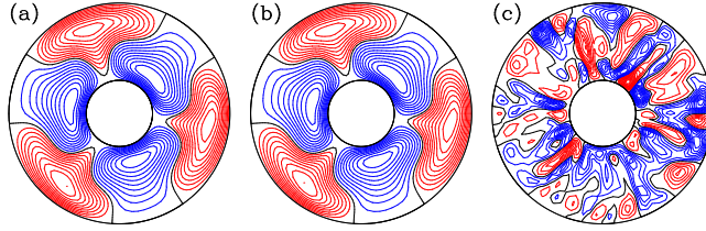
Figure 11: Contour plots of the temperature for, a) the left snapshot Fig. 9, b) its reconstruction using expansion (3.30), and c) the difference between both.
