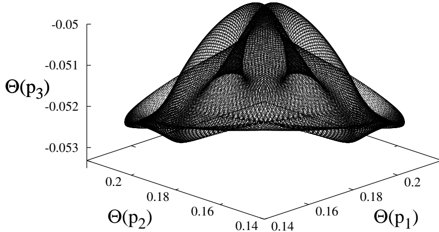
Figure 14: Three-dimensional projection of the trajectory plotted in Fig. 10. The points p_1 , p_2 , and p_3 are located at (r, \phi) with r = 1.246 , and \phi = \phi_0 - \pi/5 , \phi_0 + \pi/5 and \phi_0 .
