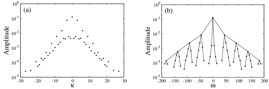
Figure 12: The (a) a - \kappa and (b) a - \omega diagrams for the quasi-periodic flow.
