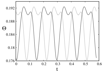
Figure 6: Counterpart of Fig. 2 for the more complex periodic flow.
