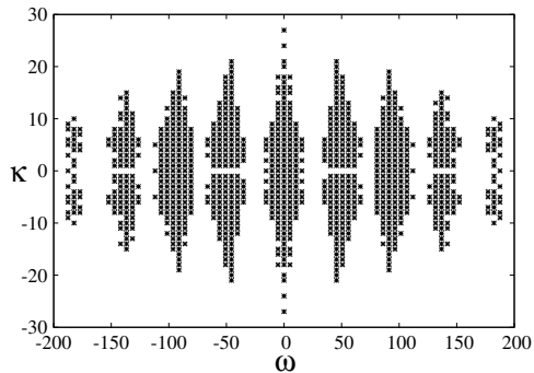
Figure 13: The \kappa - \omega diagram for the quasi-periodic flow.
