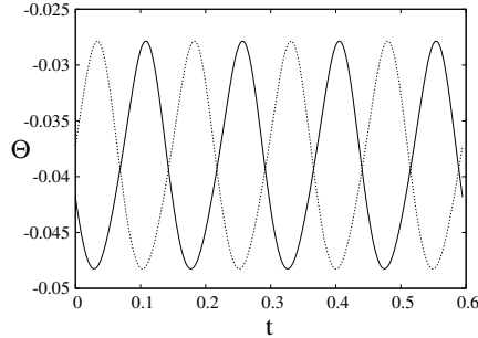
Figure 2: Time evolution of the temperature at two points symmetrically located around the thick dashed line in Fig. 1.
