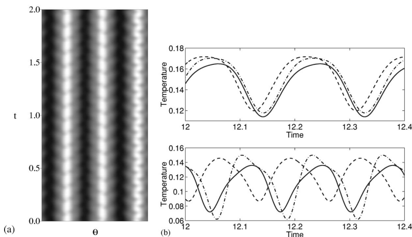
FIG. 4. (a) Shadowgraph showing the evolution of the temperature perturbation in time (y axis) at the radial midpoint of the annulus for a solution corresponding to Ra=12300 . (b) Time dependence of the temperature showing the phase shift between the three points of the annulus of coordinates (L/2, \theta + 2\pi m/3) , with m=0,1,2 and L the number of radial points.
