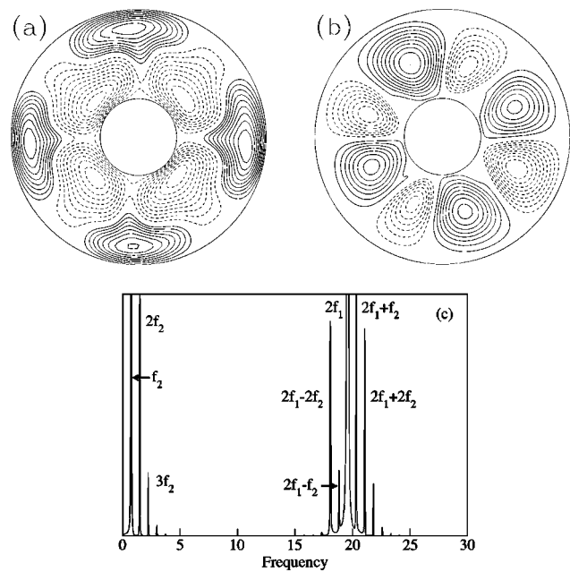
FIG. 8. For the quasi-periodic solution at Ra=18\,900 , (a) contour plots of the perturbation of the temperature, (b) of the streamfunction, and (c) Fourier spectrum of the temporal series of the Nusselt number. As in the n=3 quasi-periodic solution, the main frequency of the solution is f_1 .
