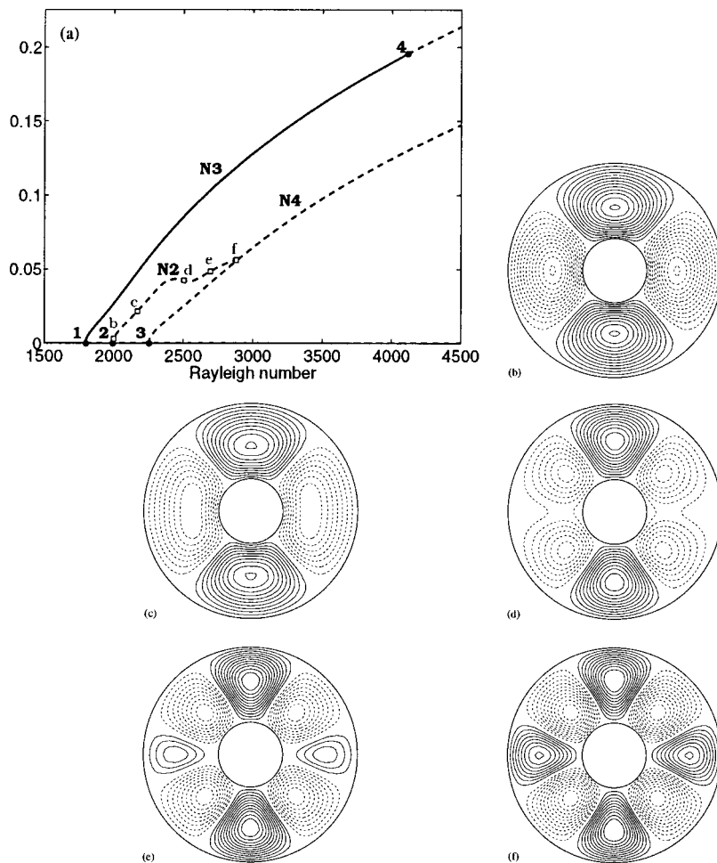
FIG. 1. (a) Bifurcation diagram showing branches of columnar modes with wavenumbers n=3 , n=2 , and n=4 ( N3 , N2 , and N4 branches, respectively). They arise at Ra_c^1=1799 (1), Ra_c^2=1995 (2), and Ra_c^3=2254 (3). (b)–(f) The contour plots of the temperature perturbation showing the structure of the solutions in the N2 branch, corresponding to the points b ( Ra=2000 ), c ( Ra=2198 ), d ( Ra=2500 ), e ( Ra=2711 ), and f ( Ra=2875 ) in the diagram, respectively.
