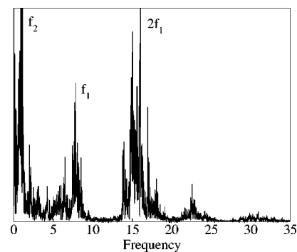
FIG. 6. Fourier spectrum of the temporal series of the Nusselt number. The solution corresponds to Ra=13\,000 on the main n=3 branch.
