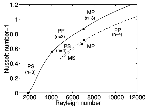
FIG. 12. Nusselt number as a function of the Rayleigh number for steady state and periodic solutions. The solid, dashed, and dotted lines correspond, respectively, to the basic n=3 , n=4 , and the mixed stable solutions. For the time-dependent solutions we have plotted the averaged period. The labels stand for: PS pure steady, PP pure periodic, MS mixed steady, MP mixed periodic solutions.
