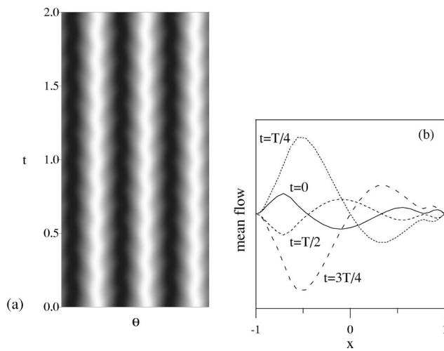
FIG. 3. Pure n=3 direction reversing traveling wave. (a) Shadowgraph showing the evolution of the temperature perturbation in time at the radial midpoint of the annulus, for a solution corresponding to Ra=5000 . (b) Four snapshots showing the radial dependence of the azimuthal mean flow.
